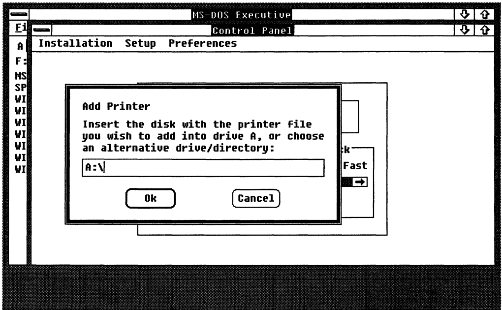
Figure 2-2 Add Printer Dialog Box
